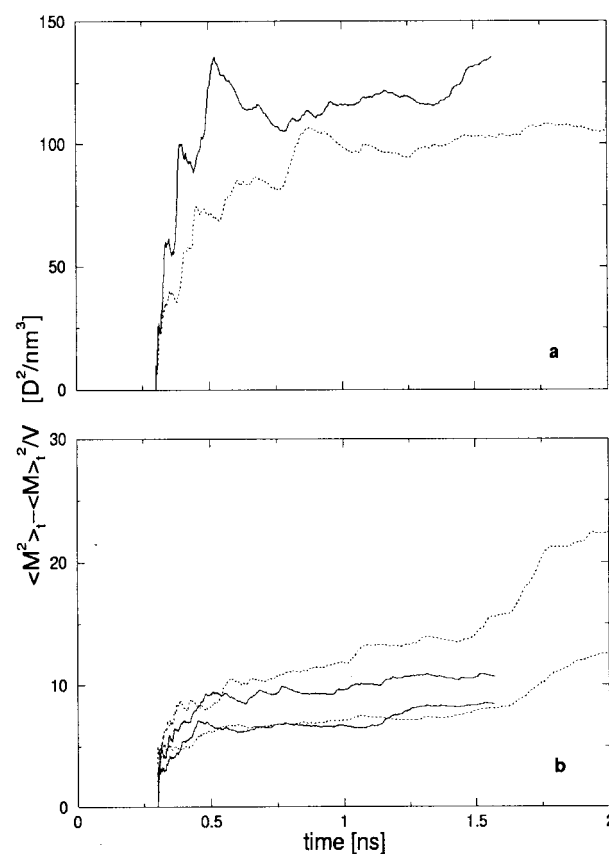
FIGURE 8 Total dipole moment fluctuation per unit volume ( \langle M^2 \rangle - \langle M \rangle^2 / V ) in units of Debye 2 /nm 3 as a function of time for the simulations of \alpha -lactalbumin ( \alpha -LAC) at pH 2.0 ( \cdots ) and pH 8.0 (—). (a) Total dipole moment fluctuation per unit volume calculated over all protein atoms; (b) Total dipole moment fluctuation per unit volume calculated for all protein atoms excluding charged residues and the charged N and C termini (upper two curves) as well as the contribution of the protein backbone only (lower two curves).
